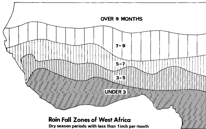
FIG. 2. Comparison of West African vegetation and rainfall zones.
