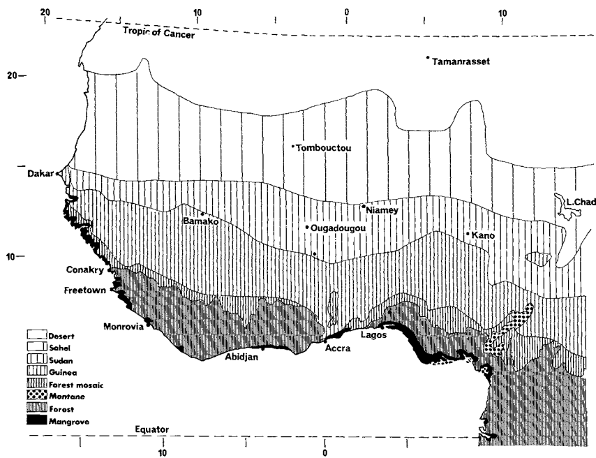
FIG. 1. Vegetation zones of West Africa.
